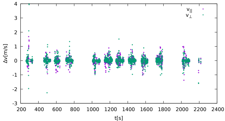
Difference between Doppler and interpolated speed (Ublox9P)
