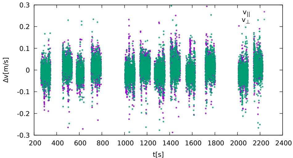
Difference between Doppler and interpolated speed (LeicaGS18)
