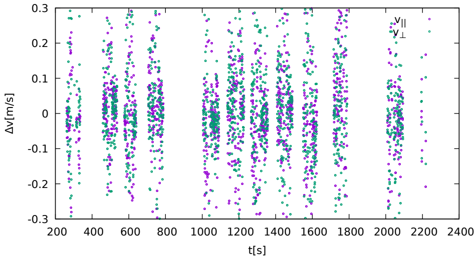
Difference between Doppler and interpolated speed (Ublox9P)
