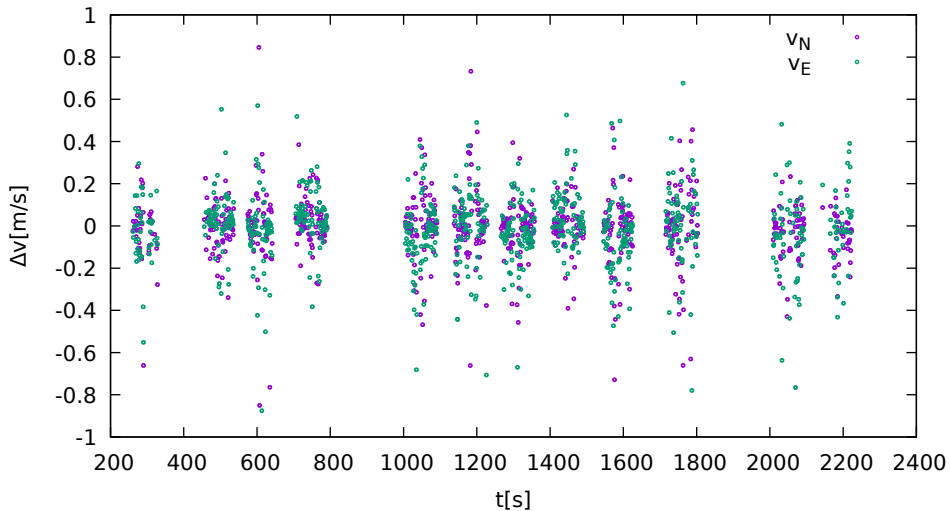
Difference between Doppler and interpolated speed (Ublox8T)
