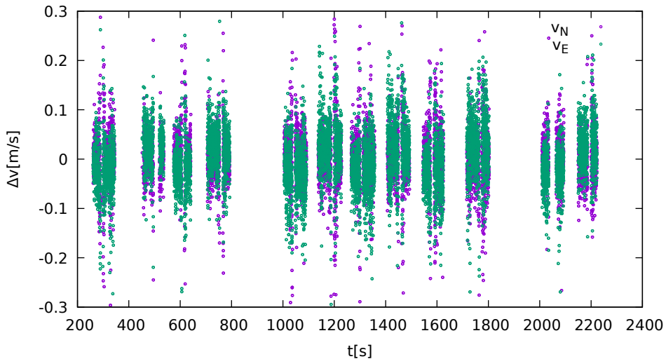
Difference between Doppler and interpolated speed (LeicaGS15)
