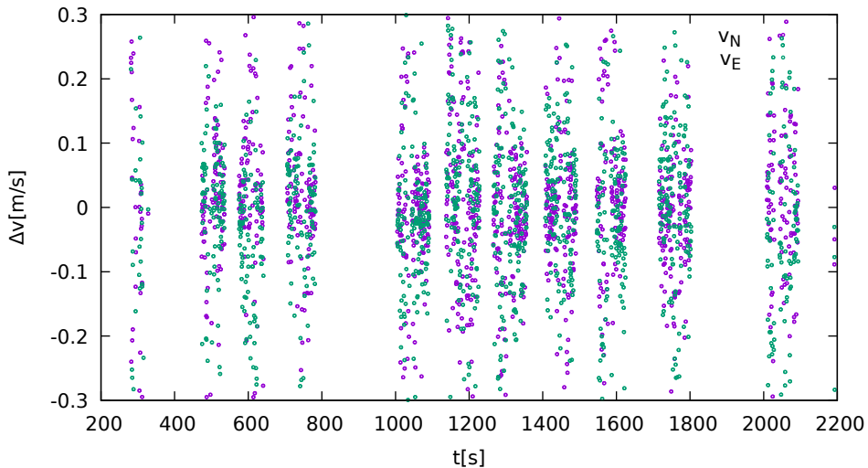
Difference between Doppler and interpolated speed (Ublox9R)
