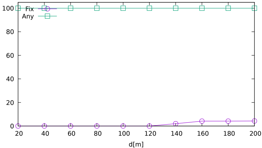
Solution ratio vs. jammer distance (Javad on GLONASS)
