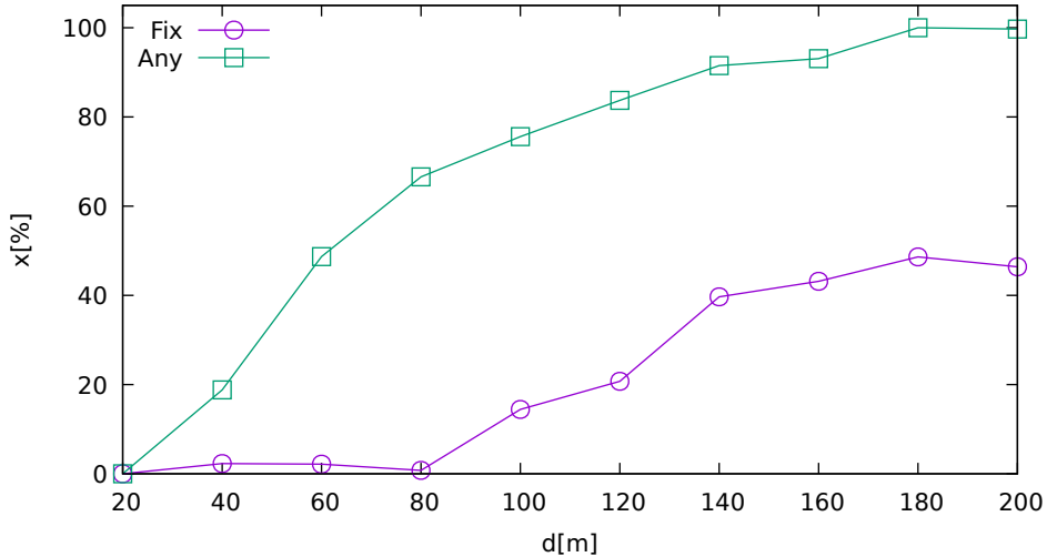
Solution ratio vs. jammer distance (Javad on GPS)
