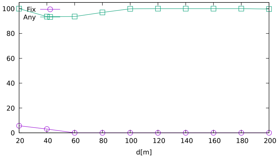
Solution ratio vs. jammer distance (Javad on GPS/GLONASS)
