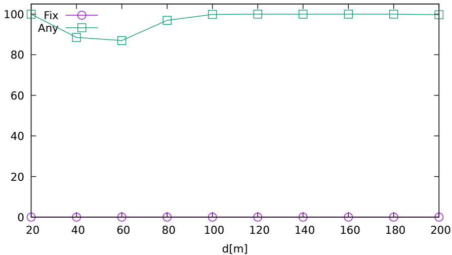
Solution ratio vs. jammer distance (Javad on GPS/GLONASS/Galileo)
