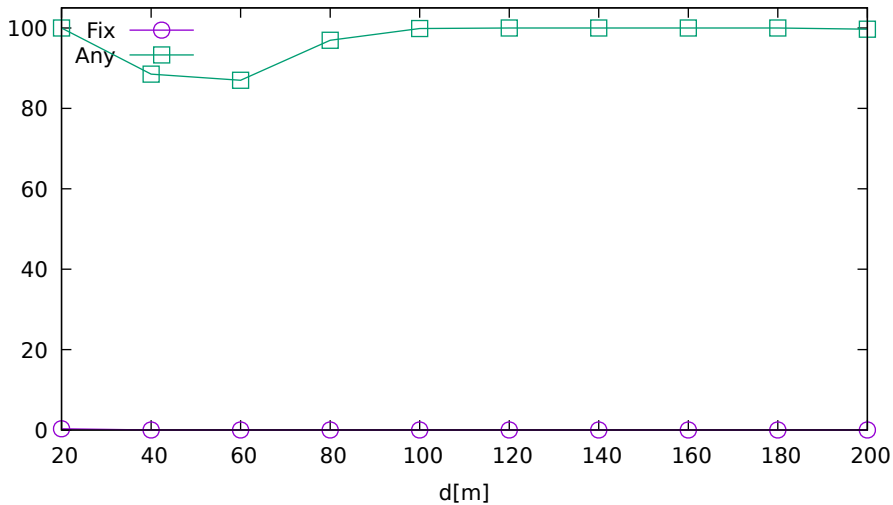
Solution ratio vs. jammer distance (Javad on GPS/GLONASS/Galileo/BeiDou)
