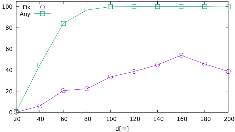
Solution ratio vs. jammer distance (Javad on GPS/Galileo)
