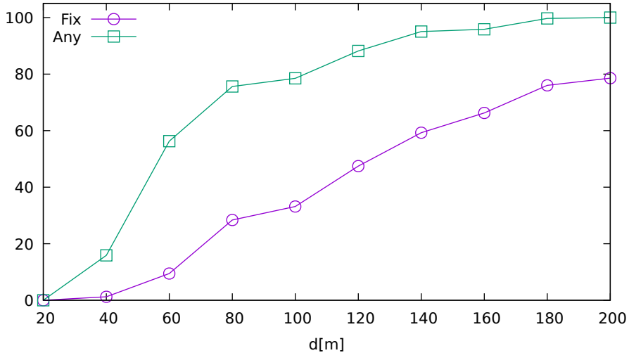
Solution ratio vs. jammer distance (Javad on Galileo)
