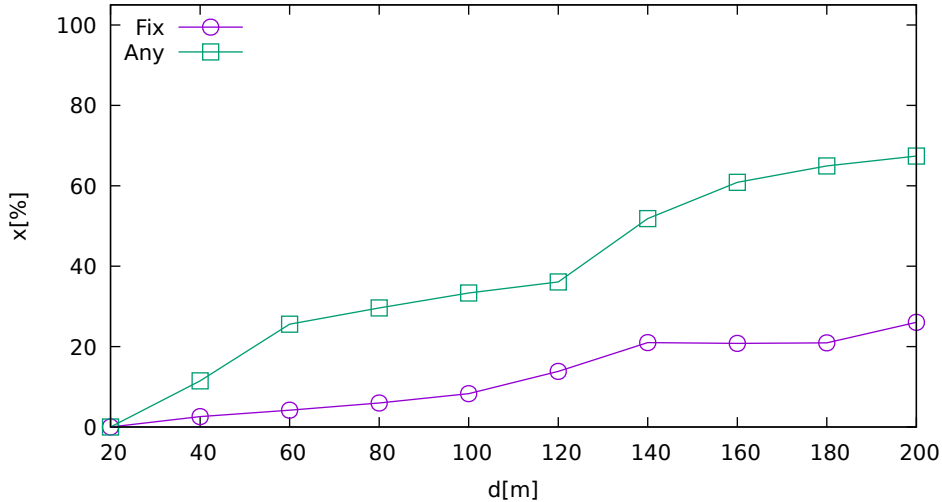
Solution ratio vs. jammer distance (LeicaGS15 on GLONASS)
