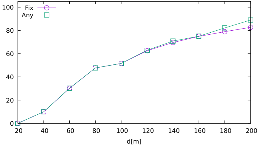
Solution ratio vs. jammer distance (LeicaGS15 on GPS)
