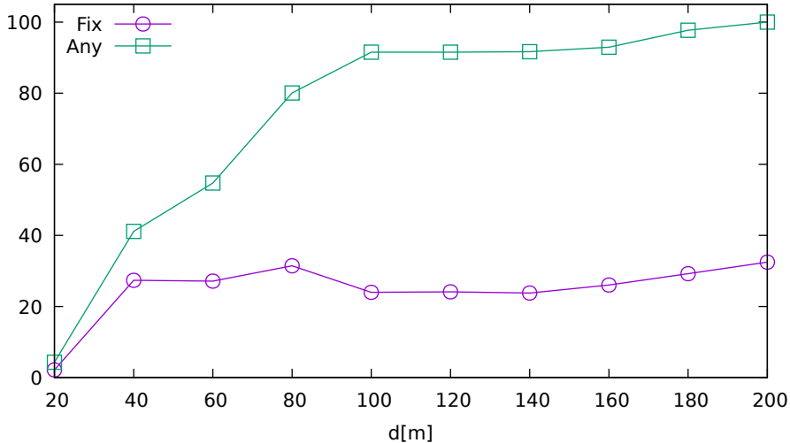
Solution ratio vs. jammer distance (LeicaGS15 on GPS/GLONASS/Galileo)
