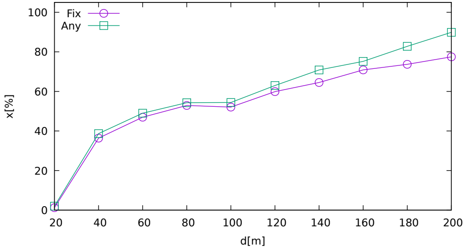
Solution ratio vs. jammer distance (LeicaGS15 on GPS/Galileo)
