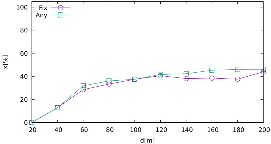
Solution ratio vs. jammer distance (LeicaGS15 on Galileo)
