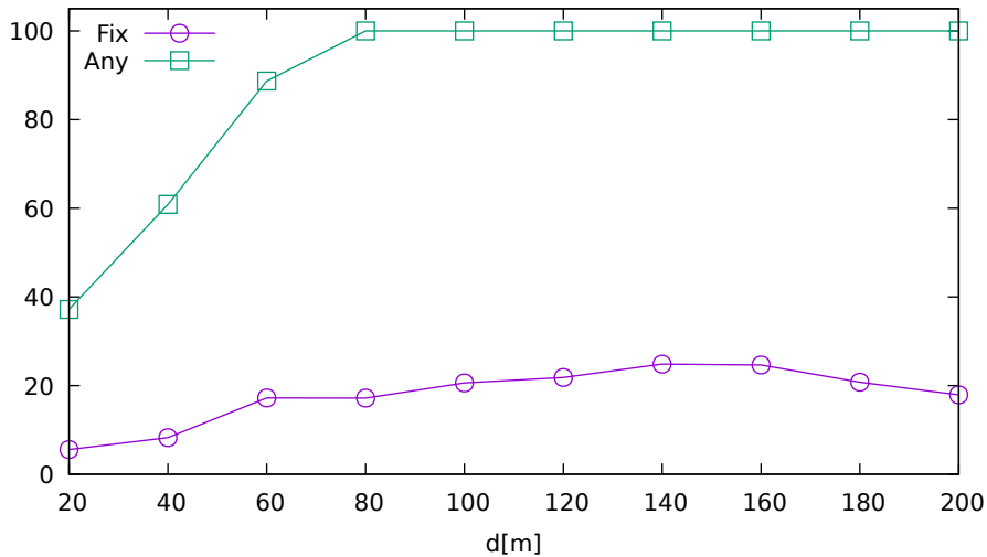
Solution ratio vs. jammer distance (LeicaGS18 on BeiDou)
