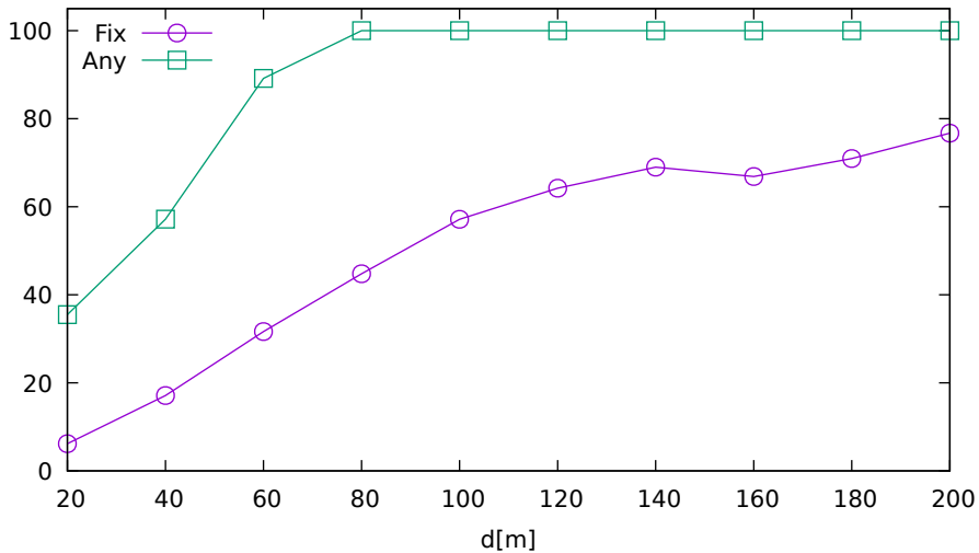
Solution ratio vs. jammer distance (LeicaGS18 on GLONASS)
