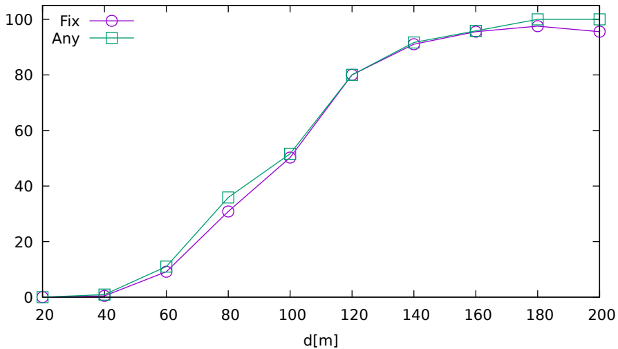
Solution ratio vs. jammer distance (LeicaGS18 on GPS)
