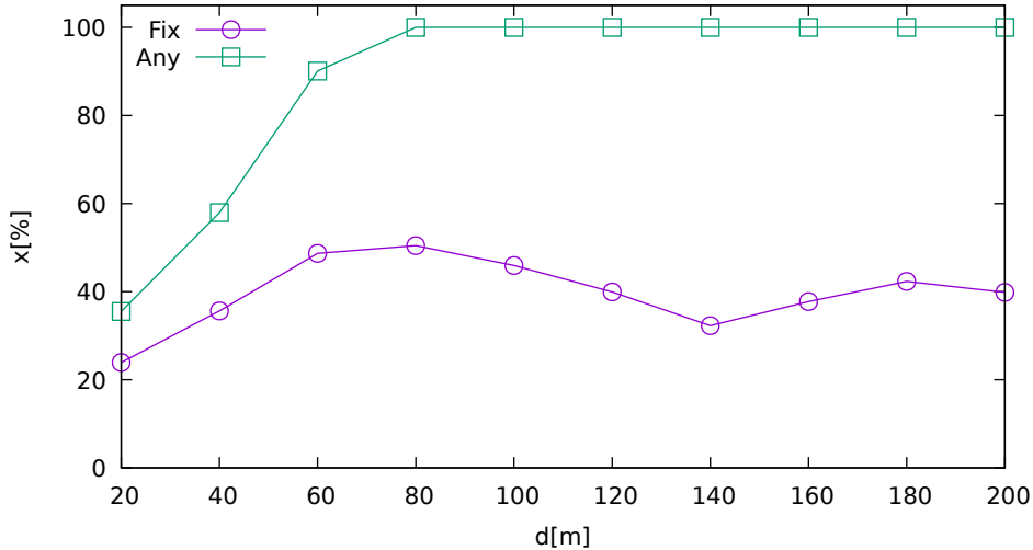
Solution ratio vs. jammer distance (LeicaGS18 on GPS/GLONASS)
