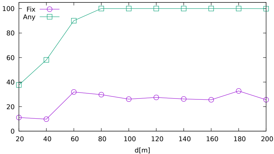
Solution ratio vs. jammer distance (LeicaGS18 on GPS/GLONASS/Galileo)
