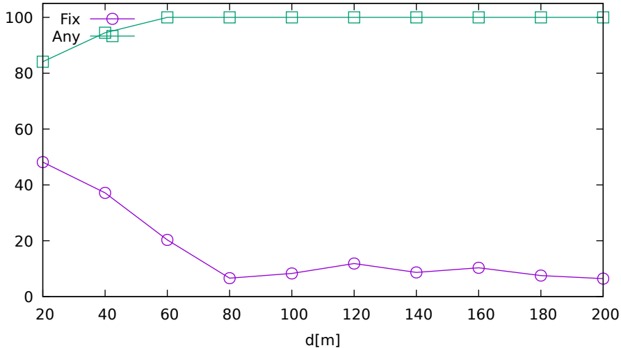
Solution ratio vs. jammer distance (LeicaGS18 on GPS/GLONASS/Galileo/BeiDou)
