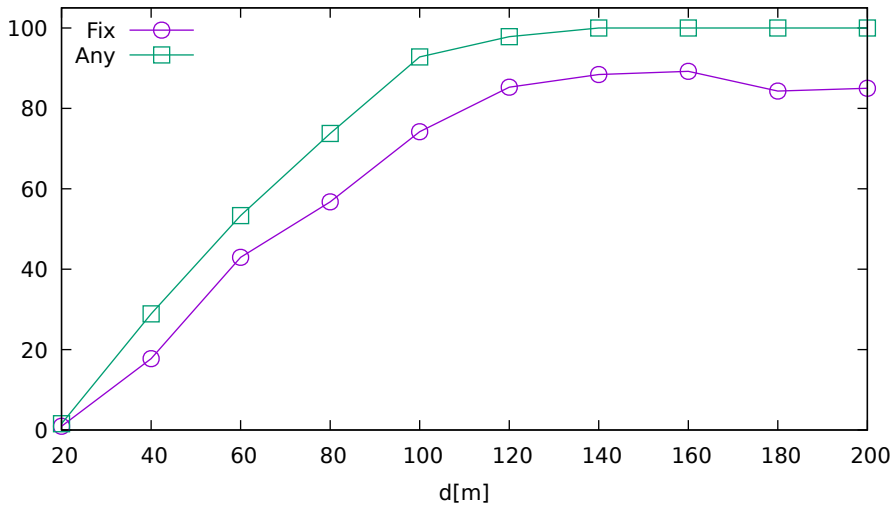
Solution ratio vs. jammer distance (LeicaGS18 on GPS/Galileo)
