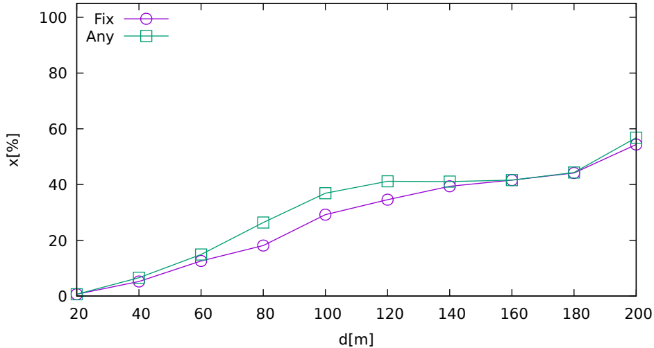
Solution ratio vs. jammer distance (LeicaGS18 on Galileo)
