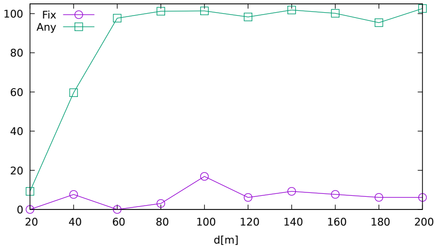
Solution ratio vs. jammer distance (Ublox8T on GLONASS)
