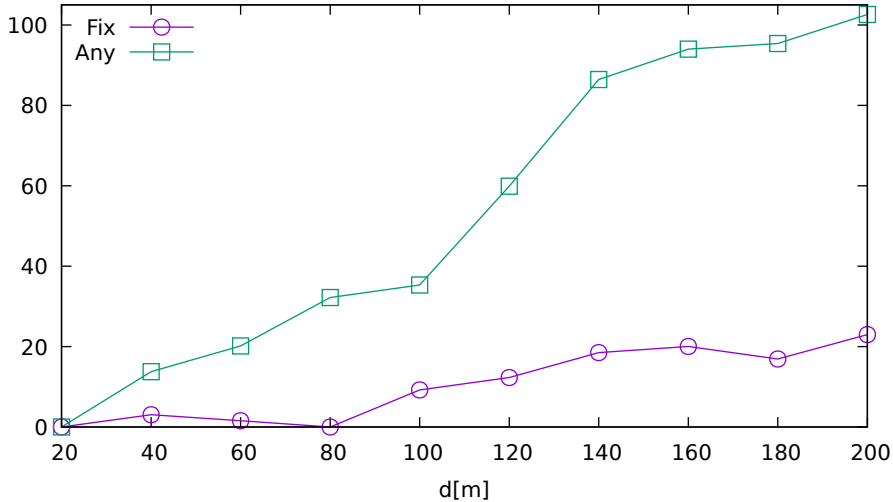
Solution ratio vs. jammer distance (Ublox8T on GPS)
