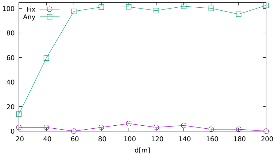
Solution ratio vs. jammer distance (Ublox8T on GPS/GLONASS)
