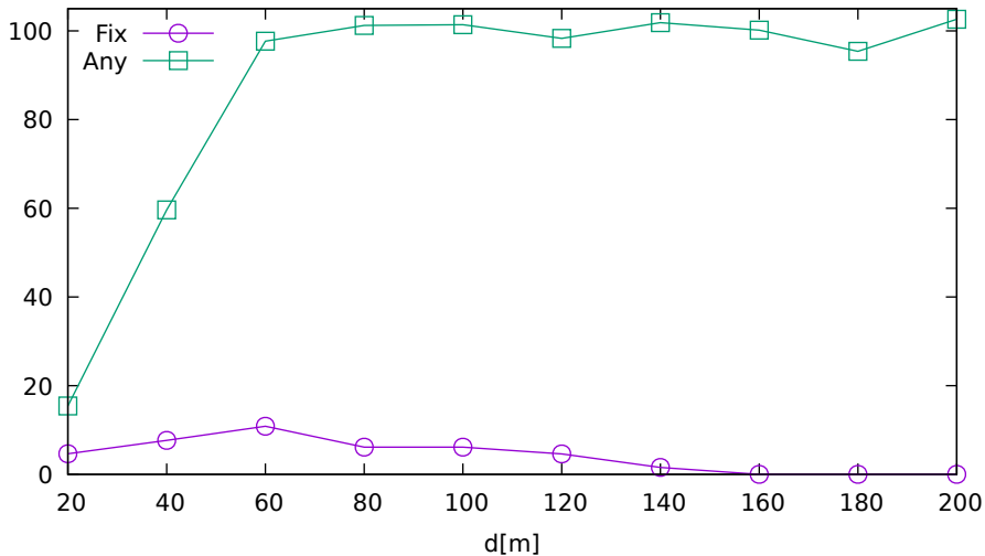
Solution ratio vs. jammer distance (Ublox8T on GPS/GLONASS/Galileo)
