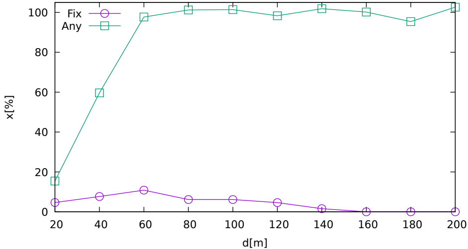
Solution ratio vs. jammer distance (Ublox8T on GPS/GLONASS/Galileo/BeiDou)
