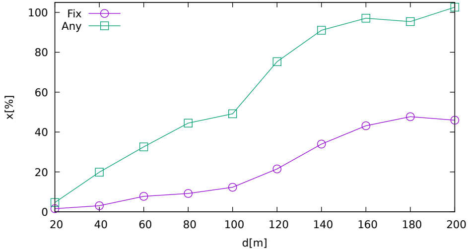
Solution ratio vs. jammer distance (Ublox8T on GPS/Galileo)
