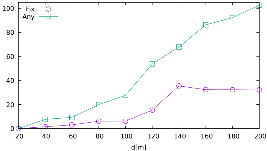
Solution ratio vs. jammer distance (Ublox8T on Galileo)
