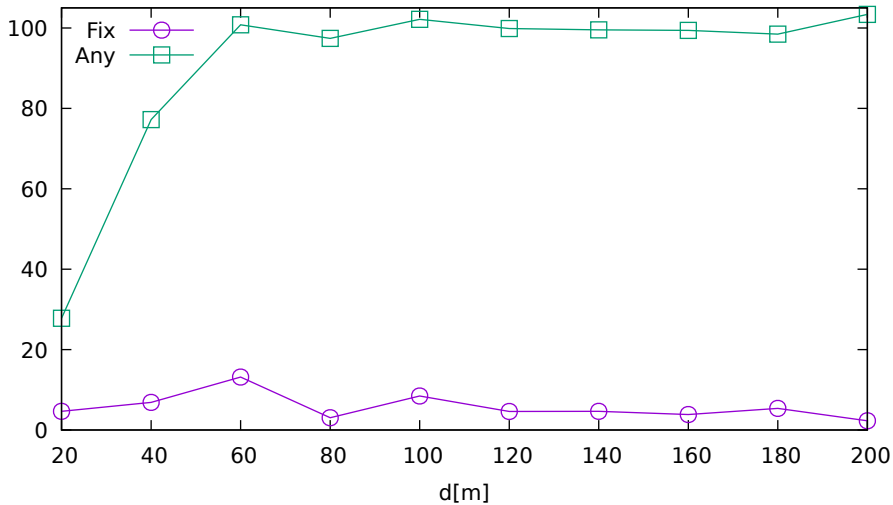
Solution ratio vs. jammer distance (UbloxF9P on BeiDou)
