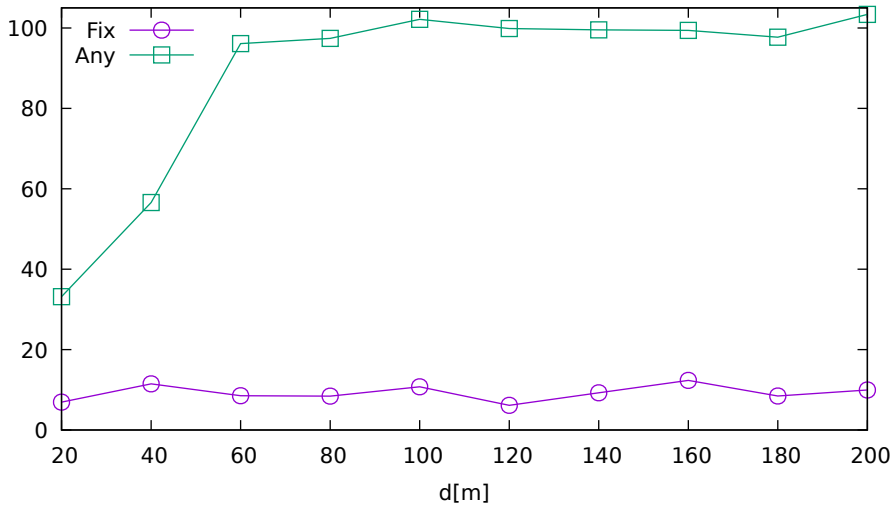
Solution ratio vs. jammer distance (UbloxF9P on GLONASS)
