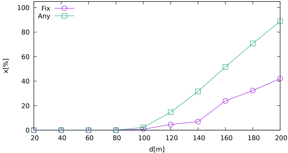
Solution ratio vs. jammer distance (UbloxF9P on GPS)
