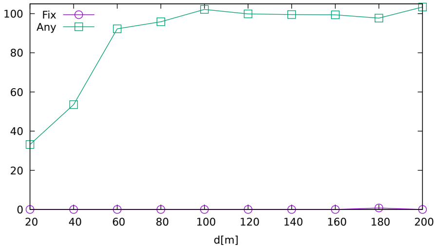
Solution ratio vs. jammer distance (UbloxF9P on GPS/GLONASS)
