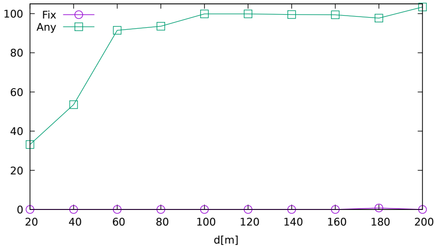
Solution ratio vs. jammer distance (UbloxF9P on GPS/GLONASS/Galileo)
