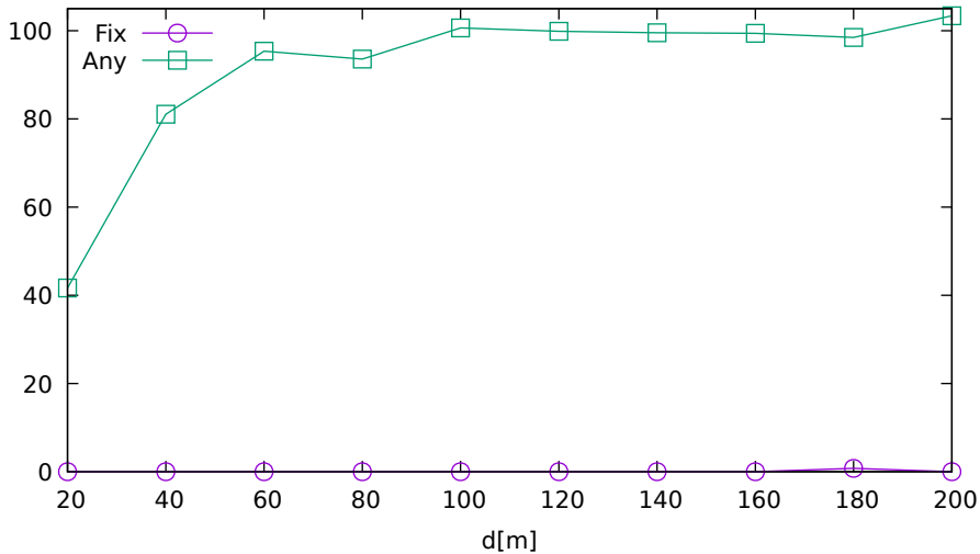
Solution ratio vs. jammer distance (UbloxF9P on GPS/GLONASS/Galileo/BeiDou)
