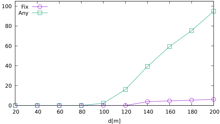
Solution ratio vs. jammer distance (UbloxF9P on GPS/Galileo)
