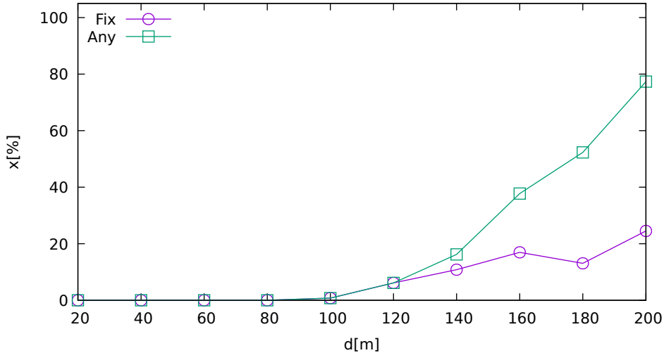
Solution ratio vs. jammer distance (UbloxF9P on Galileo)
