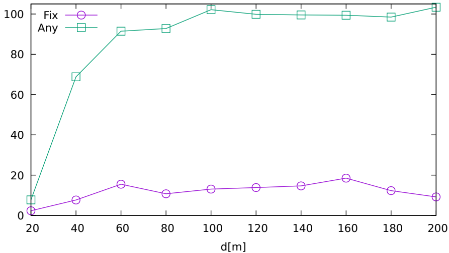
Solution ratio vs. jammer distance (UbloxF9R on BeiDou)
