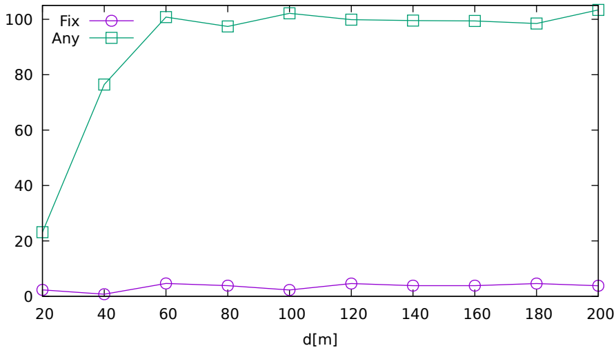
Solution ratio vs. jammer distance (UbloxF9R on GLONASS)
