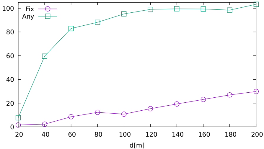
Solution ratio vs. jammer distance (UbloxF9R on GPS)
