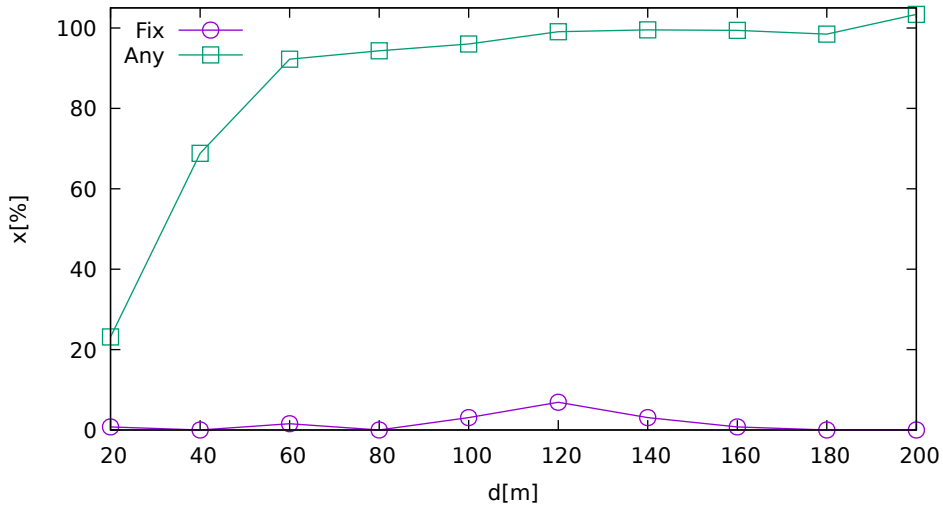
Solution ratio vs. jammer distance (UbloxF9R on GPS/GLONASS)
