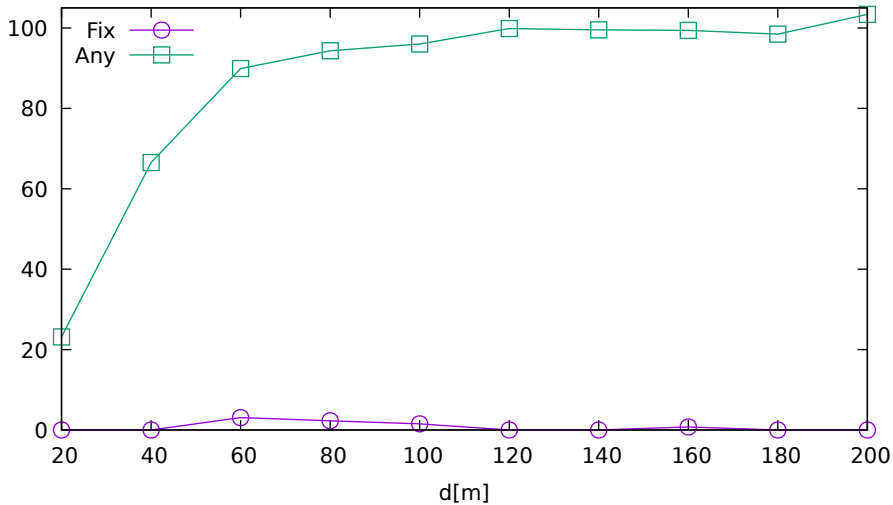
Solution ratio vs. jammer distance (UbloxF9R on GPS/GLONASS/Galileo)
