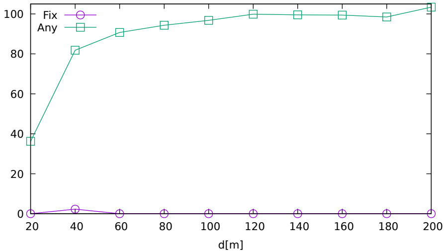
Solution ratio vs. jammer distance (UbloxF9R on GPS/GLONASS/Galileo/BeiDou)
