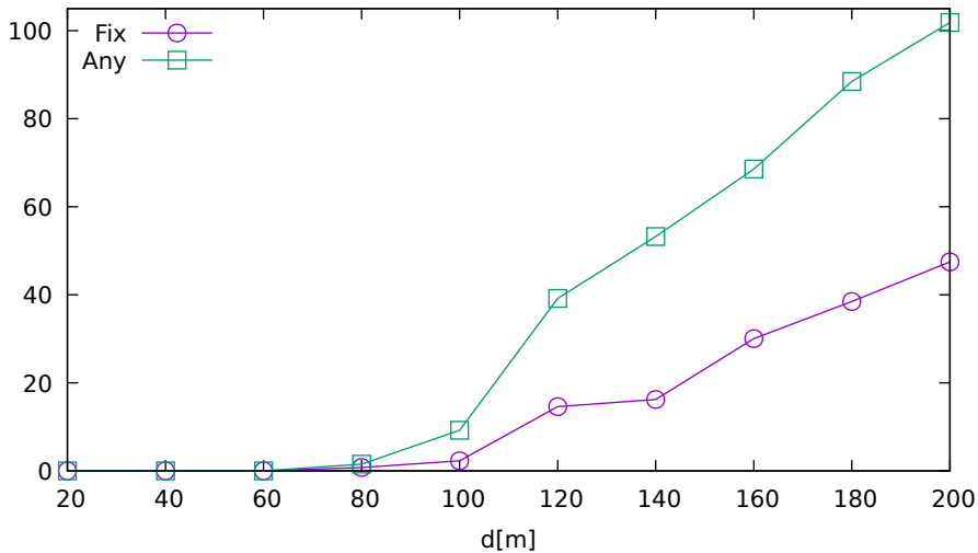
Solution ratio vs. jammer distance (UbloxF9R on GPS/Galileo)
