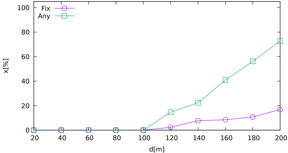
Solution ratio vs. jammer distance (UbloxF9R on Galileo)
