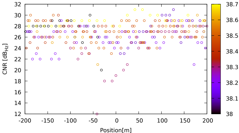
CNR vs position for C09 (B1) on HuaweiP40 - DOY 262 jam. 2
